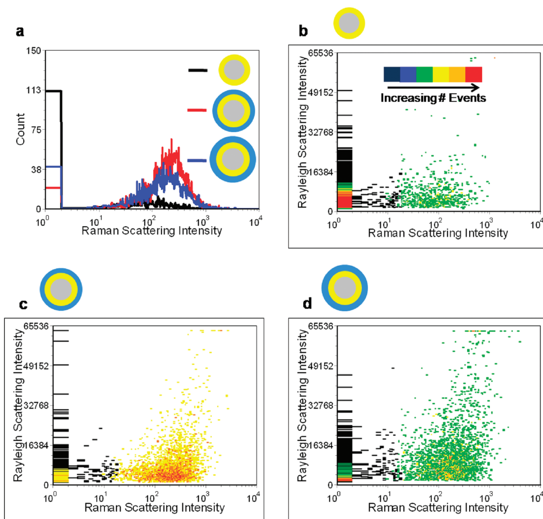
Figure 3. SERRS tag population analysis. (a) Histograms of Raman scattering intensity from three SERRS tag preparations prepared with 0, 3, and 5 \mu\text{L} of silver enhancement solution. Illustrations display the relative sizes of the silica core (gray), gold shell (yellow), and silver shell (blue). (b–d) Density plots of SERRS tags prepared with 0, 3, and 5 \mu\text{L} of silver enhancement solution. The analysis was performed using 340 mW of 647 nm excitation and signal integration times of 300 \mu\text{s} .
