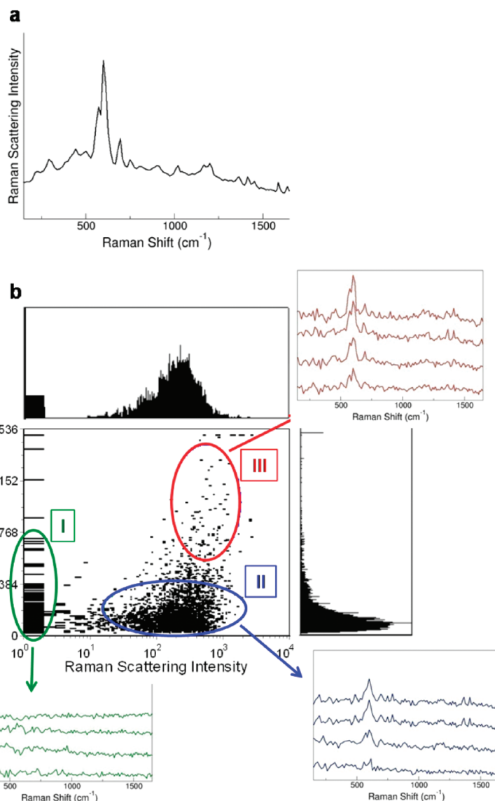
Figure 2. Ensemble and flow spectroscopy analysis of nanoshell SERRS tags. (a) Ensemble oxazine 170 SERRS tag Raman spectrum from tags prepared with 2 \mu\text{L} of silver enhancement solution. Spectrum was collected from a 0.9 pM nanoshell solution ( 5.5 \times 10^8 NPs/mL as measured using flow spectroscopy) using 14 mW of 647 nm laser excitation and a signal integration time of 2 s. (b) Univariate and bivariate displays of Rayleigh and Raman scattering intensity from single tag flow spectroscopy analysis and representative single tag spectra from each subpopulation. Spectra were collected using 340 mW of 647 nm excitation and signal integration times of 300 \mu\text{s} and have been offset for clarity.
